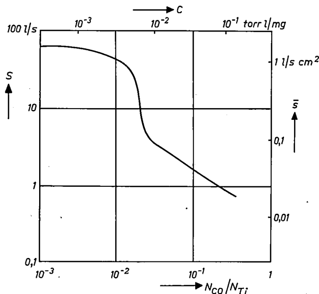
Fig. 3. Pumping speed S , in l/sec as a function of specific gettering capacity C in torr.litre/mg, calculated from the data in fig. 2; or, which is equivalent, the ratio N_{CO}/N_{Ti} between the number of gettered CO molecules and the number of titanium atoms incident on the getter surface, as a function of \bar{s} , the mean pumping speed (in l/sec) of the getter film per cm 2 .
