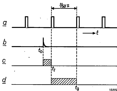
Fig. 10. a) Pulse train at the inputs 1 of flip-flops F_1 and F_2 in fig. 9. b) "Display" pulse at input 2 of F_1 , produced when button B is depressed. c) During the interval t_0-t_1 , F_1 is in state II . d) During the interval t_1-t_2 (= duration of one frame) F_2 is in state II . The recording amplifier A_2 (fig. 9) is then unblocked and the picture is recorded on the wheel.
