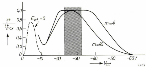
Fig. 7. Illustrating the effect which the negative potential V_{CC'} (on the side plates C and C') has on the ion current i^+ . V_R = 0.15 V; V_{hf} = 1 V rms ; i^- = 1 \mu A; B = 0.5 Wb/m 2 .
