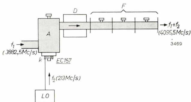
Fig. 12. Circuit for an EC 157 used as a mixer to produce a frequency shift of the RF signal in the straight-through relay station shown in fig. 3. LO local oscillator. Other symbols as in fig. 11.
