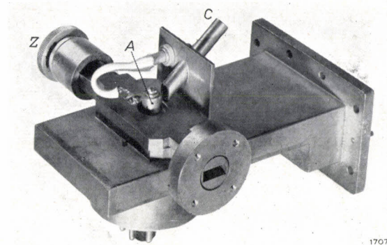
Fig. 7. Frequency multiplier stage equipped with an EC 157 triode, capable of producing 20 000 Mc/s by multiplying 4000 Mc/s. A anode. C nozzle for cooling-air supply. Z knob for adjusting tuning plunger. Driven by about 1 W at 4000 Mc/s the available power at the output is approx. 0.1 mW at 20 000 Mc/s.
