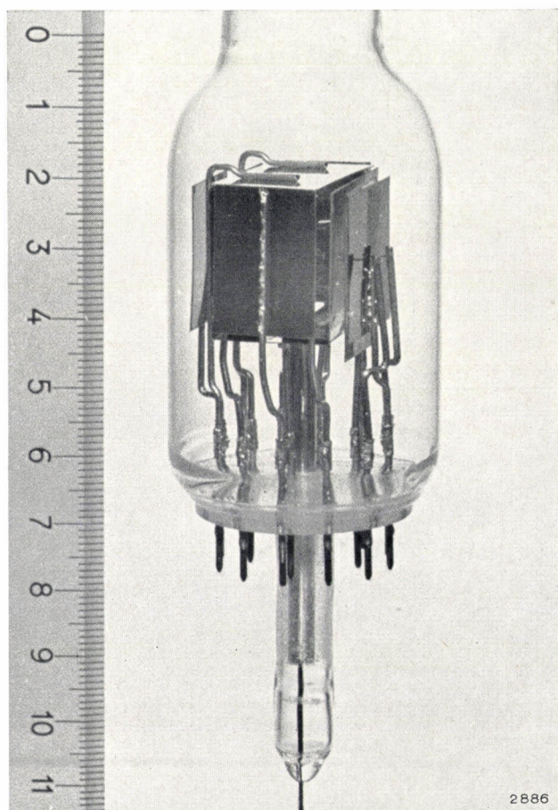
Fig. 4. The omegatron, with rings and side plates, in a glass envelope. The cathode is on the right, and on the extreme left is the collector for the electrons which have traversed the omegatron. The ions formed in the space inside the omegatron move to the ion collector. This is connected to the central metal pin fused into the glass tube.
