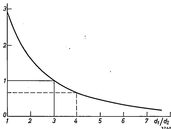
Fig. 4. Hull and Burger correction graph 3) for comparing measurements on bead seals having different ratios of bead diameter d_1 and wire diameter d_2 . A result obtained for d_1/d_2 = 4 is divided by 0.7 to reduce it to the result for d_1/d_2 = 3 .
