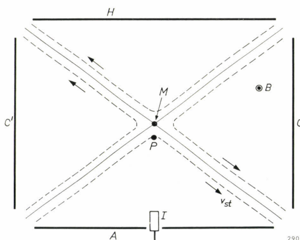
Fig. 5. Cross-section of omegatron perpendicular to the direction of the magnetic field. M is the electrical centre, P the position where the ions are formed. I ion collector. A and H electrodes to which the RF voltage is applied. C and C' side plates, which are given a negative potential with respect to A and H . The dashed lines represent equipotential lines.
