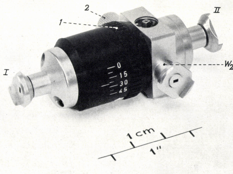
Fig. 20. Rotary directional coupler for 2 mm waves. I , II and W_2 as in fig. 18a. 1 rotatable ring for twisting the polarization strip; the angle of twist \alpha is read from the scale. 2 knob for adjusting the plunger in W_2 . Directivity >25 dB, standing-wave ratio <1.16 .
