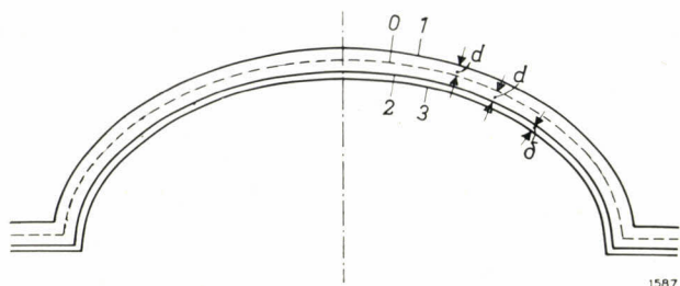
Fig. 5. Curve 0 is the calculated meridian curve of the geometrical surface possessing the required properties. Curves 1 and 2, at a distance d ( < \frac{1}{2}\lambda ) at either side of 0, are meridians of the metal surfaces to be made. Curve 3 lies at a further distance \delta , equal to the thickness of the sheet metal used. 1 and 3 are the meridians of the jigs in which the metal sheeting will be stamped into the appropriate shape. (For clarity, the distances d and \delta are exaggerated in comparison with the other dimensions.)
