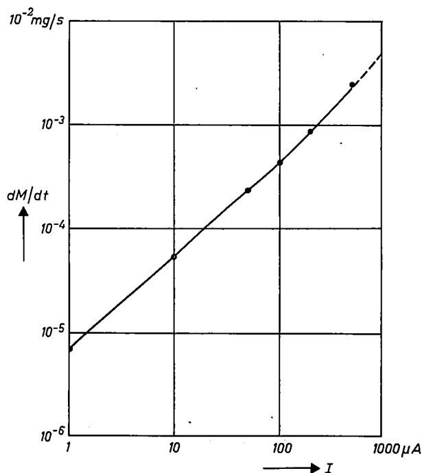
Fig. 4. Evaporation rate dM/dt in mg/sec of one cathode in the getter ion-pump, as a function of the discharge current I in μA.
