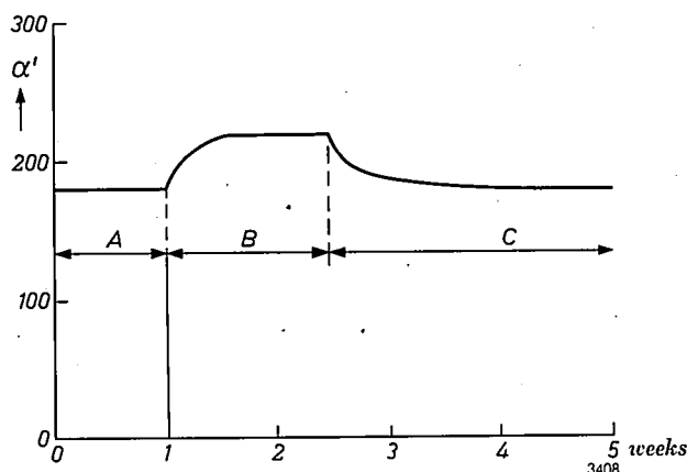
Fig. 17. Transistors formed at 140 °C, with powdered arsenic mixed in the silicone grease, often show a marked "shelf after-effect".
