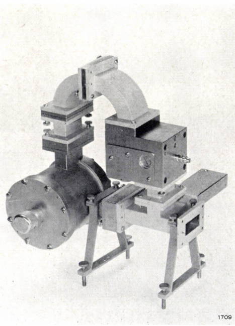
Fig. 9. a) Oscillator for 4000 Mc/s fitted with an EC 157, built on the principle of fig. 8a. b) Similar oscillator, but for 6000 Mc/s and fitted with a 5 cm, 1 W triode. Both oscillators, a and b , are reproduced on the same scale.
