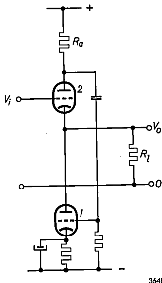
Fig. 15. Basic diagram of a cathode follower consisting of two valves in cascade. If the two valves are pentodes, the gain differs very little from unity and is largely independent of the valve characteristics. Moreover, the input impedance is very high since no grid leak is needed, the cathode follower being directly coupled to its probe and thus biased to the potential of the probe, which differs little from zero.
