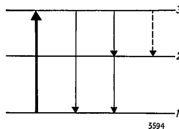
Fig. 5. Illustrating the operation of a solid-state maser, after Bloembergen. A paramagnetic salt is used whose ground state in a magnetic field splits into at least three levels.
