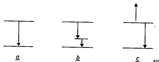
Fig. 4. Recombination processes.
