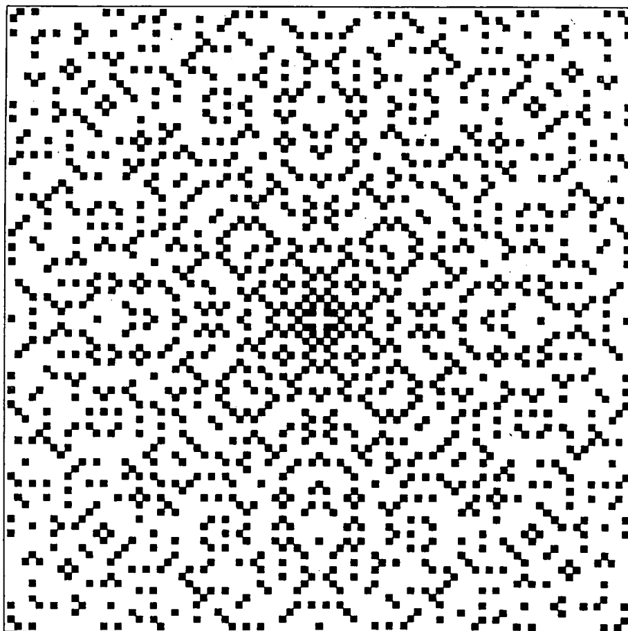
Fig. 12. The black squares represent in the complex plane (with origin in the centre) the complex prime numbers of Gauss, i.e. the numbers (m + jn) that cannot be written as m + jn = (a + jb)(c + jd) , where m, n, a, b, c, d are integers. This pattern was woven into a fabric marketed by an Eindhoven textile factory.
