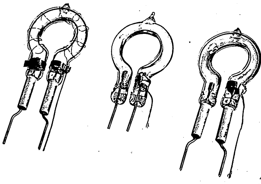
Fig. 11. Three types of trigger electrode for electronic-flash lamps; from left to right: trigger wire wound around the tube; strip of conductive material (not distinctly visible, owing to reflections in the glass); transparent conductive layer (not visible). The latter type has certain advantages.
