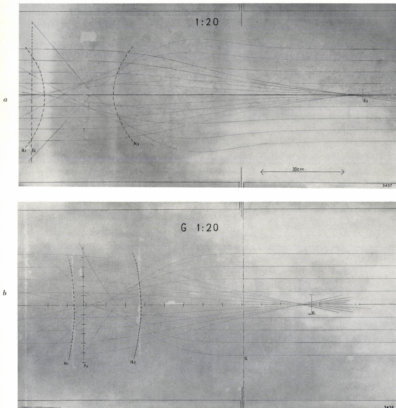
Fig. 17. a ) Electron trajectories as traced out by the automatic plotter for the model of an accelerating lens. (The electrodes of this model are shown in fig. 1.) The lens consists of two adjacent coaxial cylinders of the same diameter; the potential with respect to earth of the right cylinder is 20 times that of the left one. The trajectories are drawn in a plane through the axis of the lens. The electrons enter parallel to the axis, from the left and also from the right. The principal planes and focal planes are indicated, together with the situation of the electrodes.
