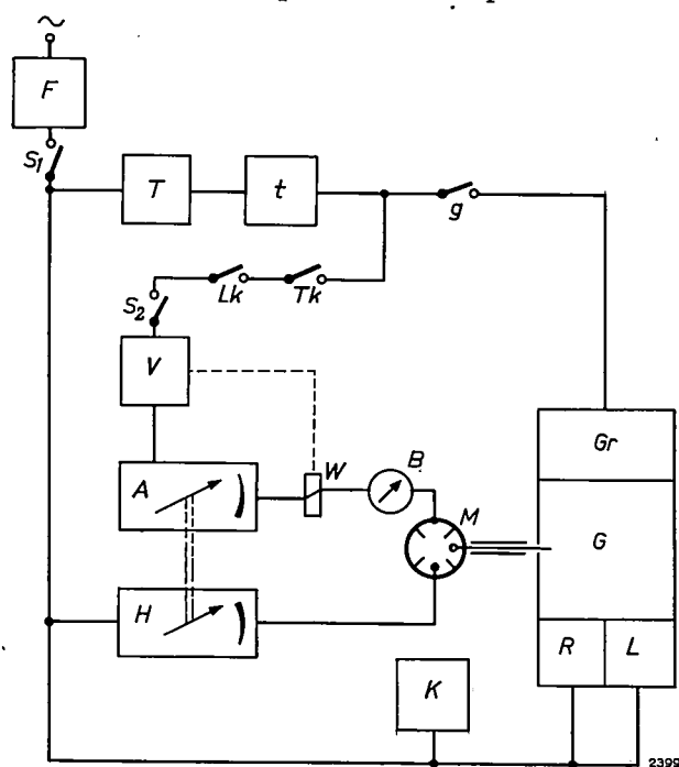
Fig. 10. Block diagram of a microwave cooker. F suppressor filter. S_1 main switch. T time relay. t timer. S_2 switch for magnetron high tension. Lk and Tk safety switches, which can close only when the magnetron temperature is not too high and the oven door is closed. V anode-voltage switch. A power pack supplying anode voltage. H filament-current transformer. W overload safety device. M magnetron. B ammeter for anode current. K cooling fan for magnetron. G oven. R field stirrer. L air extractor. Gr grill element. g switch for Gr .
