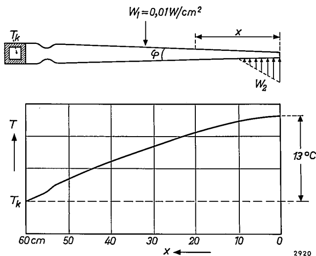
Fig. 19. Variation of temperature T over the profile of a tuning-fork blade, calculated by treating the profile as a straight truncated wedge with a constriction at the stem of the tuning fork. From the outer surface a power W_1 ( = 0.01 \text{ W/cm}^2 ) goes inwards, and from the inner surface a power W_2 (at the position of the stator). The foot of the tuning fork is kept at the temperature T_k by a cooling-water pipe.
