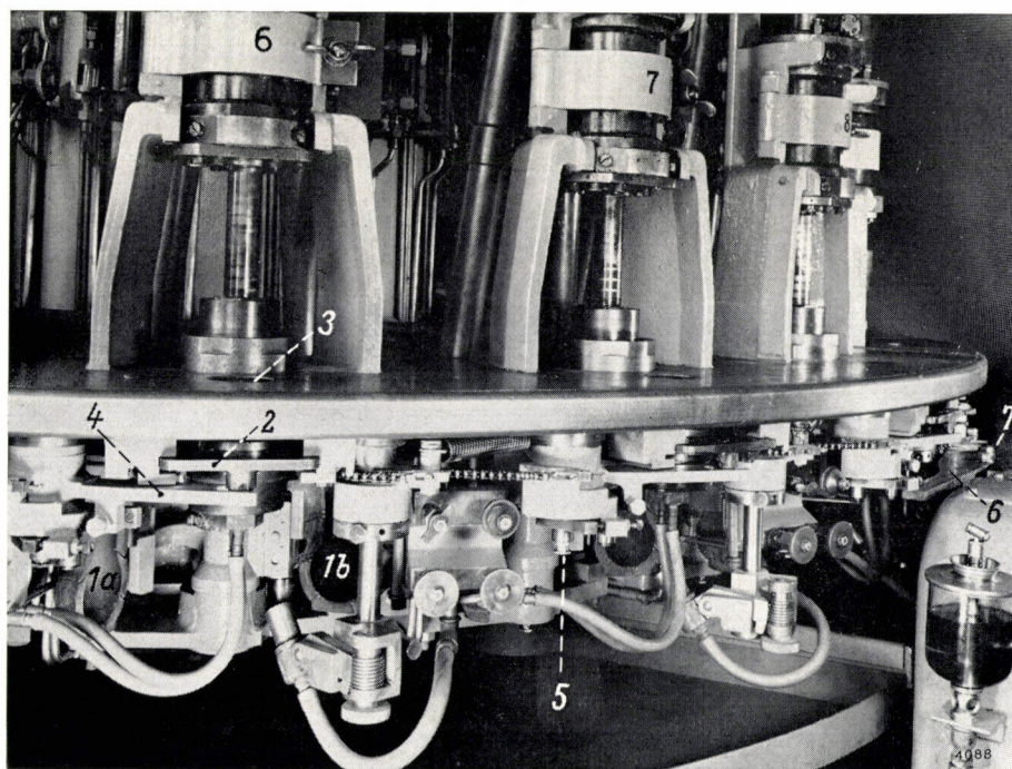
Fig. 8. Detail of the machine in fig. 9 . Among the components that can be identified are the two mating halves of a blow-mould, 1a and 1b , and the slide 2. As soon as a gob has fallen through the hole 3 into the tray, the slide is pushed inwards by the lever 4, the forked end of which engages a roller. This lever is itself turned on a spindle by a cam 6 (extreme right of photograph) on the cross-beam 7. (The relevant spindle in one of the neighbouring blow units is indicated by the figure 5.)
