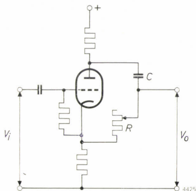
Fig. 10. One of the two cascade stages forming the phase shifter. When the resistance R is varied from zero to R_{\max} , the phase angle \alpha between output voltage V_o and input voltage V_i increases from zero to 2 \tan^{-1} \Omega CR_{\max} , that is, to nearly \pi if \Omega CR_{\max} is large compared with unity. Since there are two stages in cascade, the total phase shift runs from zero to nearly 2\pi . The magnitude of V_o is not thereby affected.
