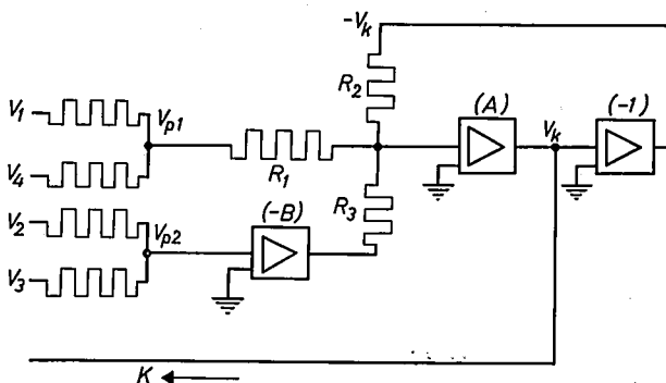
Fig. 14. Principle of the computing circuit for V . This circuit ensures that the potential at the point midway between the probes always remains zero. The resistances and gain figures A and B are chosen such that V_k = -V ; the inverting amplifier delivers the voltage V .
