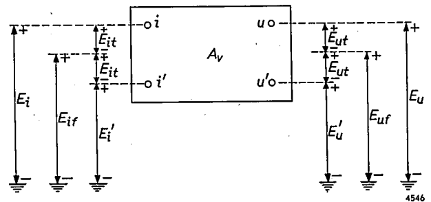
Fig. 10. Difference amplifier A_v , with input voltages E_i and E_i' , and output voltages E_u and E_u' . Also indicated are the in-phase components E_{if} and E_{uf} and the anti-phase components E_{it} and E_{ut} of these voltages.
