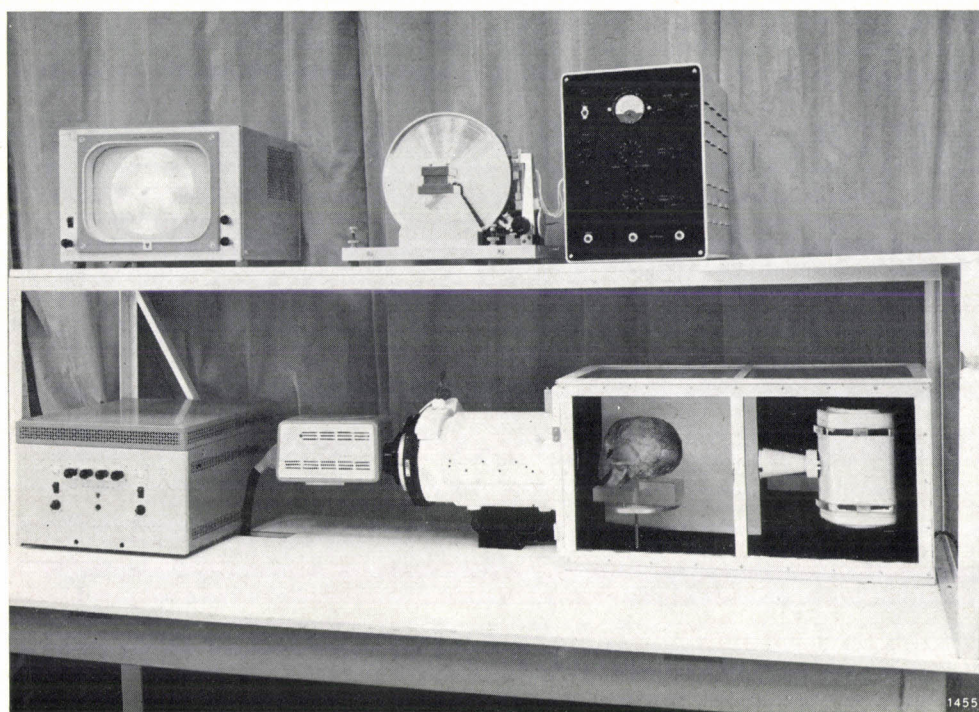
Fig. 16. Equipment for demonstrating the radio-logical application of the magnetic wheel store (as yet without frequency modulation). From right to left, below: X-ray tube, subject (a skull), X-ray image intensifier, television camera, auxiliary apparatus for television system; above: amplifying apparatus for recording and reproduction, magnetic wheel, monitor.
