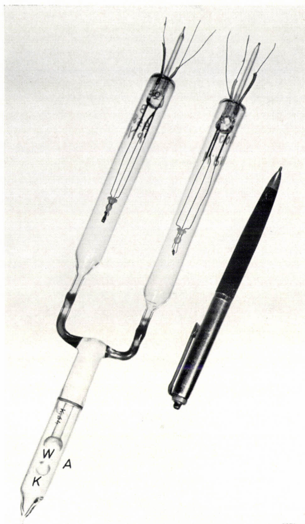
Fig. 7. Glass apparatus for admitting pure water vapour to vacuum-dried transistors. The marble K is used to break the spherical partition W which seals off the space A containing water. The water-vapour pressure is regulated by the temperature of space A (provided this temperature is lower than that of the space in which the transistor is situated). The apparatus here contains a P-N-P and an N-P-N transistor, for the purpose of comparing the behaviour of the two types.
