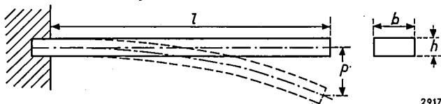
Fig. 7. Uniform bar clamped at one end. The width b of the cross-section is irrelevant to considerations concerning the amplitude p , the frequency f_m and the bending stress \sigma .
