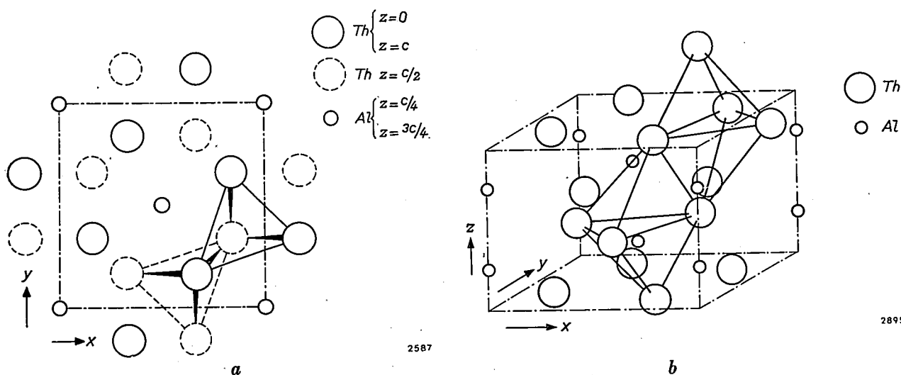
Fig. 8. The unit crystal cell of \text{Th}_2\text{Al} , a substance with gettering properties. The thorium atoms form tetrahedrons, a number of which are shown. Absorbed gas atoms or ions take up positions in the interstices of these tetrahedrons. a) Projected positions of the atoms looking along the c axis (5.86 Å). The levels of the various atoms ( z ) are given in fractions of the c axis. The x and y directions are those of the a and b axes, respectively (both 7.62 Å). b) Perspective view of unit cell, showing atomic positions. The x , y and z directions are again the a , b and c axes.
