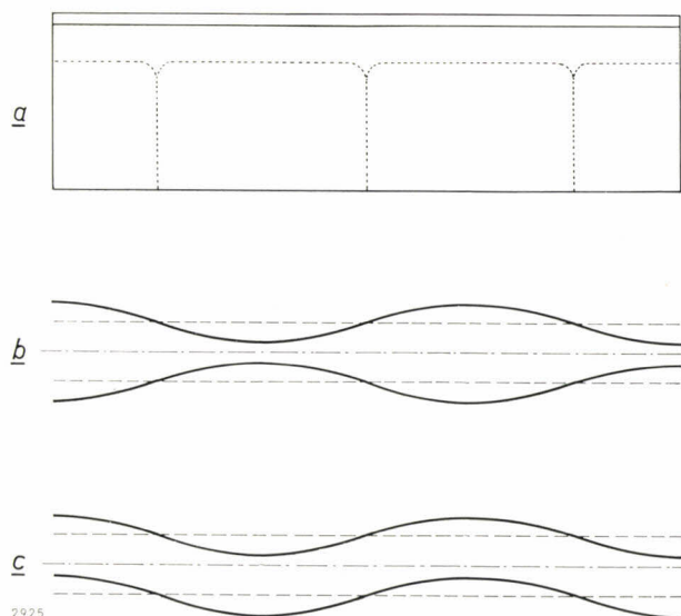
Fig. 16. a ) Chladni's figure of a vibration of the tuning fork, with three nodes at the front edge and none at the sides of the blades (except the fundamental node as in fig. 10 ). The two blades can vibrate here in two modes: symmetrically ( b ), called the s03 mode; or anti-symmetrically ( c ), mode a03 .
