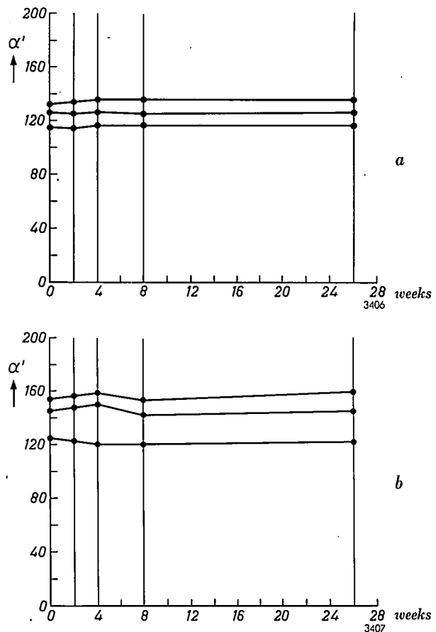
Fig. 16. Some examples of the constancy of \alpha' of transistors formed with arsenic. Before each measurement of \alpha' , the transistor was shelf-stored at room temperature for 24 hours. a) During operation; dissipation 50 mW, ambient temperature 50 °C. b) Stored, at 140 °C.
