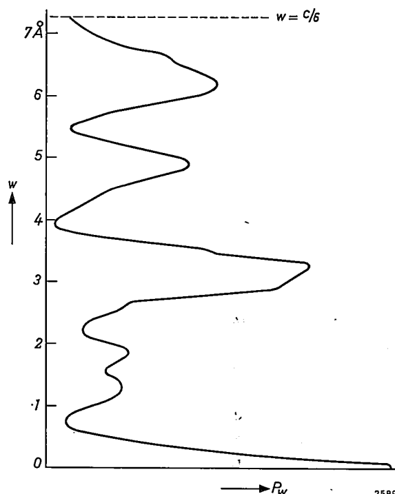
Fig. 9. Patterson plot of a one-dimensional Patterson synthesis P(w) carried out with reflections from Y-Ba 2 Zn 2 Fe 12 III O 22 . The w direction is that of the c axis. The various peaks provide information on the projections of the interatomic distances on the c axis. The peak at 3.2 Å indicated a projected spacing of that amount between barium atoms. This indication made it possible to build the first, provisional model.
