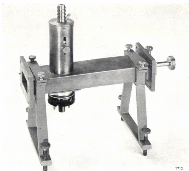
Fig. 10. Experimental oscillator with an EC 157 triode, with which frequencies up to about 8000 Mc/s are reached by using the \frac{3}{4}\lambda mode of oscillation of the anode resonant cavity.
