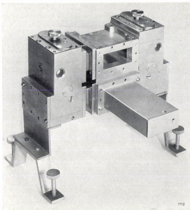
Fig. 20. Complete frequency modulator, built on the principle of fig. 17, using the block shown in fig. 19. The feedback paths of the two triodes are unequal in length and in part common. When the waves in the triodes are amplitude-modulated in push-pull, the output signal will be frequency-modulated.
