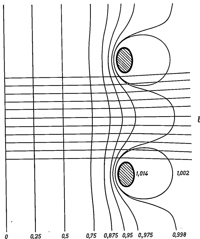
Fig. 16. The electron trajectories and equipotential lines in the field of a planar triode with an intersecting-"wire" gauze grid. (These are drawings copied from the plotted trajectories.) a) The plane in which the trajectories are drawn cuts the gauze parallel and perpendicular to the directions of the "wires". b) The plane cuts the gauze diagonally.
