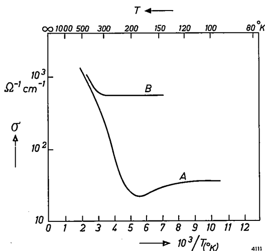
Fig. 3. Variation of conductivity of (A) P -type and (B) N -type InSb with temperature. For higher temperatures the material becomes intrinsic which is indicated by the fact (as in fig. 2) that curves A and B approximate to the same line.
