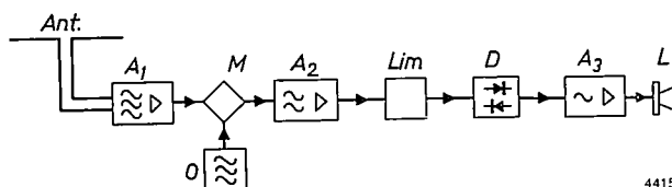
Fig. 1. Block diagram of a conventional FM broadcast receiver. Ant aerial. A_1 radio-frequency amplifier. M mixer. O local oscillator. A_2 intermediate-frequency amplifier. Lim limiter. D FM detector (discriminator). A_3 audio-frequency amplifier. L loudspeaker. (For clarity the limiter is shown as a separate block; in reality, limiting occurs partly in the last stage of A_2 , partly in the discriminator.)
