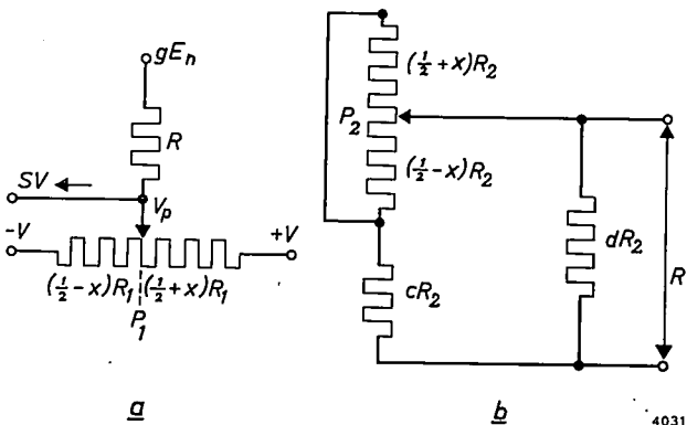
Fig. 9. a ) Principle of the steering circuit mounted on the trolley. The potentiometer P_1 is supplied with the voltages V and -V , and the resistor R with the voltage gE_n . The position of the potentiometer wiper arm is determined by the angular position of the steering shaft. The voltage V_p of the wiper is applied to the servo amplifier SV . b ) Circuit which ensures that R depends according to a certain function on the position of the steering shaft, whereby V_p is zero when the steering shaft is in the correct position. The wiper arm of potentiometer P_2 is coupled mechanically to that of potentiometer P_1 in ( a ).
