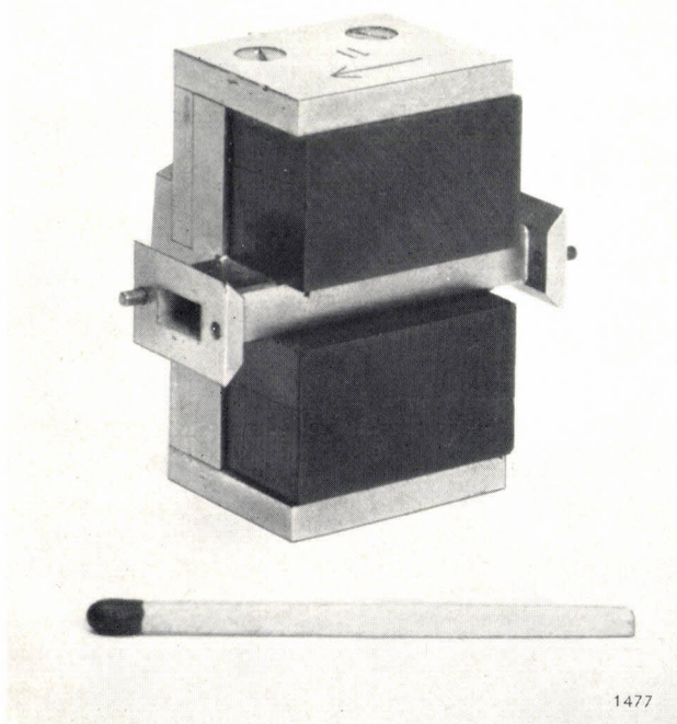
Fig. 3. Isolator for 8.6 mm waveband, using controlled uniaxial anisotropy ferrite material (anisotropy field 85 \times 10^4 A/m) and a weak external magnetic field ( 18 \times 10^4 A/m). This field is generated by a permanent magnet consisting of two blocks of ferroxdure in an iron yoke.
