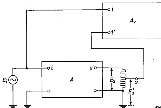
Fig. 8. Schematic representation of a method for measuring the distortion in an amplifier A , using a difference amplifier A_v .
