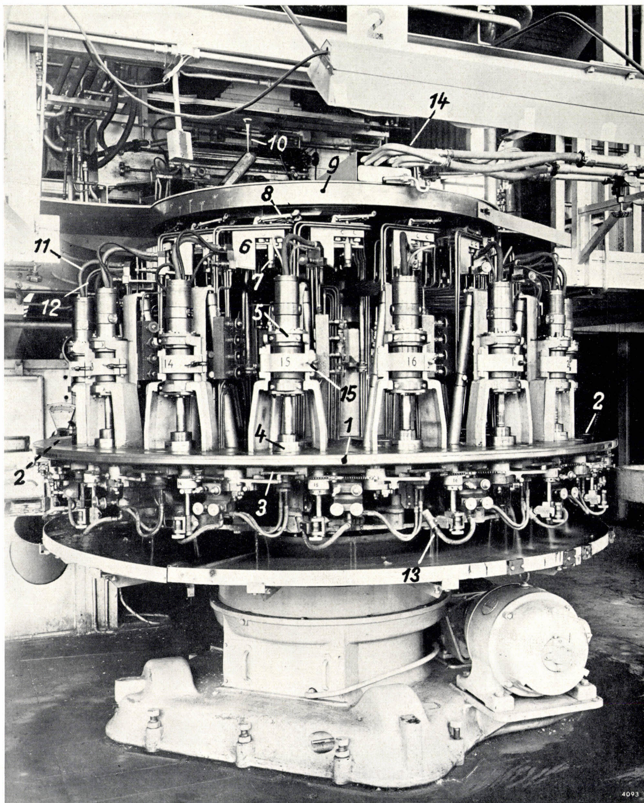
Fig. 9. Machine for making electric-lamp bulbs, equipped with 16 blowing units. 1 turntable on which the blowing units are mounted. 2 holes in the turntable through which the gobbs fall into the receiving trays. These trays are mounted in slides 3. 4 blow-head in blowing position (in which case the blow-head projects under the turntable). 5 cylinder with plunger. 6 end of a cross-beam carrying control valves. 7 outer valve of the eight carried on one cross-beam. 8 rocker arm which operates this valve. 9 cam plate. 10 stream of molten glass flowing from
