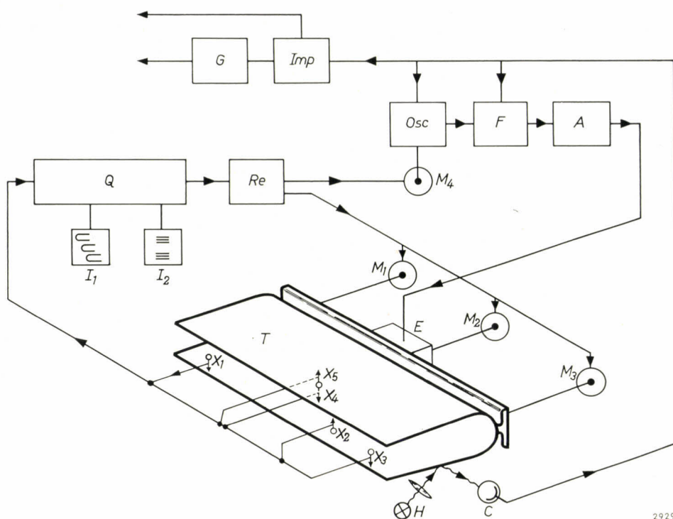
Fig. 25. Diagram of the system for automatically controlling the position and amplitude of the tuning fork. X_1 - X_5 feelers fitted to the stator for sensing the situation of the tuning fork. Q "translator", which sets in operation the appropriate combination of the four servomotors M_1 - M_4 via a series of relays Re , thereby operating the linkage for correcting the situation. I_1 and I_2 visual indicators. The three motors M_1 - M_3 act on the suspension of the tuning fork T ; M_4 acts on a potentiometer which controls the amplitude of the drive mechanism E . Osc RC oscillator, F phase-regulating circuit, and A amplifier for the drive system. H electric bulb and C photocell, which produce the feedback signal for frequency control in the drive system. This signal also serves for synchronizing the pulse generator Imp , which controls the RF generator for the cyclotron and (via G ) the ion source and irradiation set-up.
