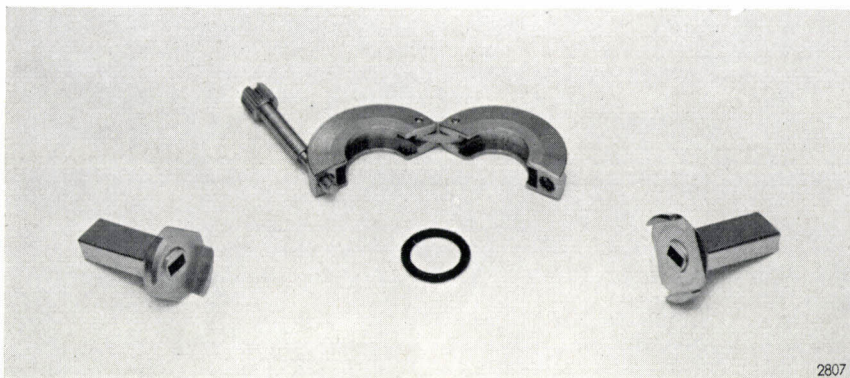
Fig. 9. Left and right, sections of waveguide with claw flanges; top centre, the hinged clamping ring which joins the flanges together; below, a rubber ring. (True size.) The clamping ring is tightened round the flanges with a single screw, perpendicular to the axis of the waveguide. The rubber ring ensures an airtight seal; the air in the whole waveguide system can then be put under pressure to prevent the entry of moisture.
