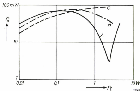
Fig. 13. The EC 157 as a limiter: output power P_o as a function of input power P_i . Anode voltage 200 V, anode current 10 mA. Curve A : amplifier not neutralized, curve B : partly neutralized, and curve C : completely neutralized.
