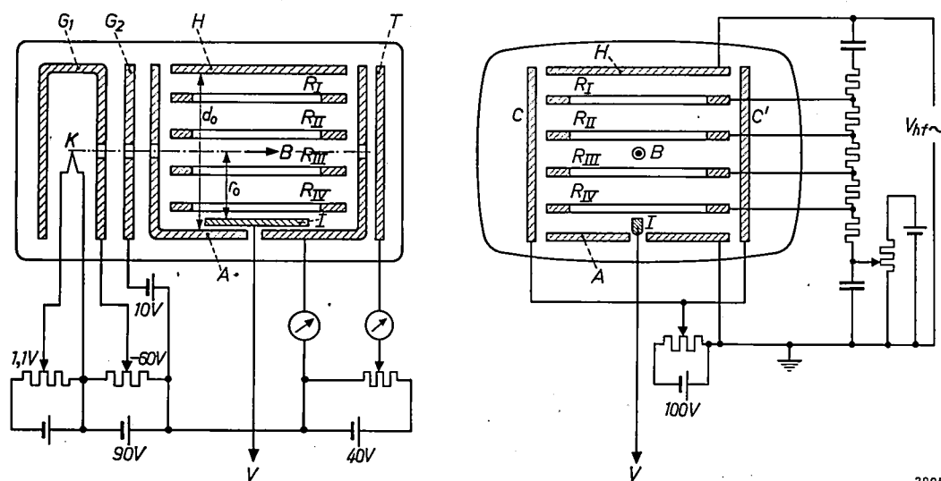
Fig. 2. Schematic representation of omegatron with rings R_I - R_{IV} and side plates C - C' . The left part of the figure shows the section parallel to the magnetic field, the right half a section perpendicular to the magnetic field (induction B ). K - G_1 - G_2 electron gun. T electron collector. I ion collector. The RF voltage is applied between the electrodes A and H . Other potentials are applied to the electrodes as indicated in the figure. The amplifier is connected at V .
