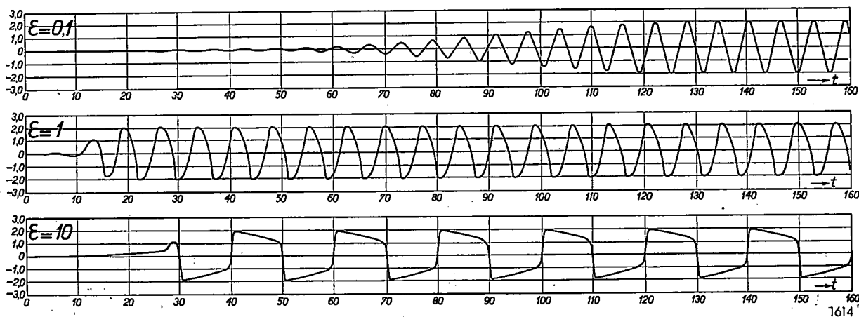
Fig. 5. Solutions of the differential equation (4), obtained by integration from solutions of eq. (5), for \varepsilon = 0.1 , \varepsilon = 1 and \varepsilon = 10 . (The variable along the abscissa, wrongly denoted by t , is the reduced quantity x .)
