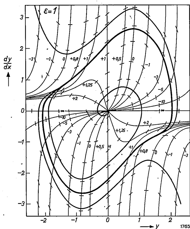
Fig. 4. Illustrating the isocline method of solving the differential equation (5), for \varepsilon = 1 .
