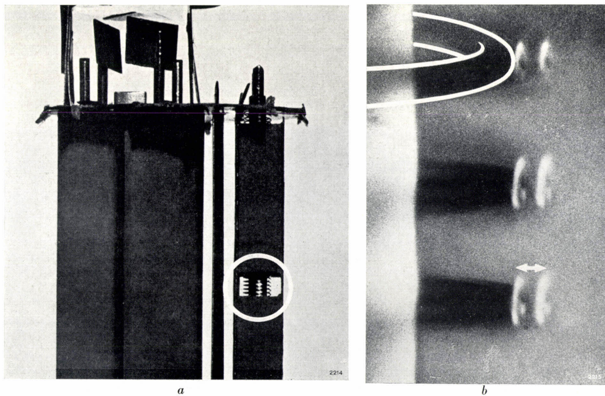
Fig. 17. a ) Electrode system of a triode-hexode. The circle marks the grid of the triode portion, visible through a hole cut into the anode. b ) Picture of the grid vibrating at its resonance frequency of 1900 c/s.
