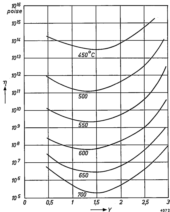
Fig. 8. Viscosity of Na_2 - K_2O - MgO - CdO - ZnO silicate glasses, at various temperatures, as a function of Y (equimolar quantities of the various metal oxides). Owing to the presence of intermediates ( Mg^{++} , Cd^{++} , and Zn^{++} ions) the calculated value Y_c , plotted here, is not the same as the actual value Y_r (which is unknown) and will be smaller. Hence the fact that the slopes of curves reverse their sign at a lower value than Y = 2 .
