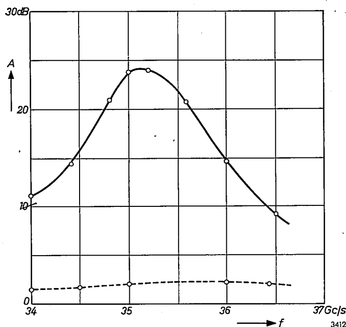
Fig. 8. Transmission characteristics of the resonance isolator without external field. The attenuation ratio here reaches a maximum of 12.
