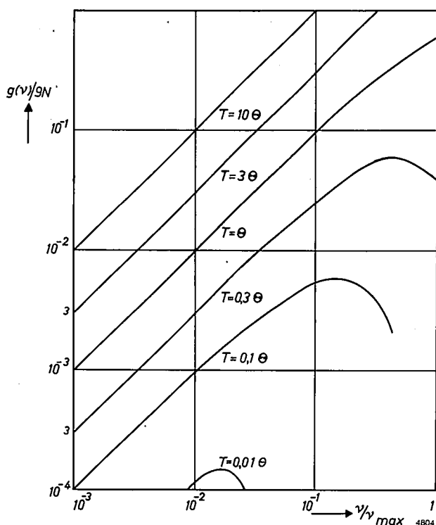
Fig. 1. The phonon spectrum in a solid. The number of phonons g(v) of frequency v (disregarding a factor 9N ) is plotted versus frequency for various temperatures. The temperature T is expressed in the figure as a fraction of the Debye temperature \Theta , the frequency as a fraction of the maximum frequency v_{\max} .
