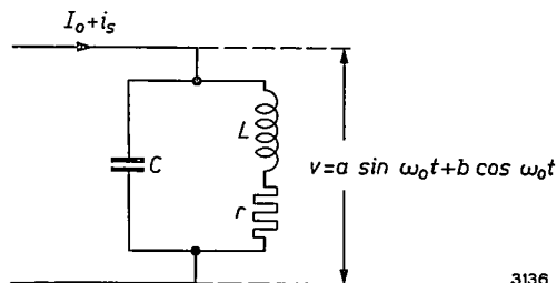
Fig. 3. The interfering current (see fig. 2) is applied to an LCr circuit. The voltage v over the circuit has the average frequency \omega_0 = 1/\sqrt{LC} , but is subject to amplitude and phase fluctuations. The voltage v may be written as the sum of a sine and a cosine component of varying amplitude a and b , respectively.
