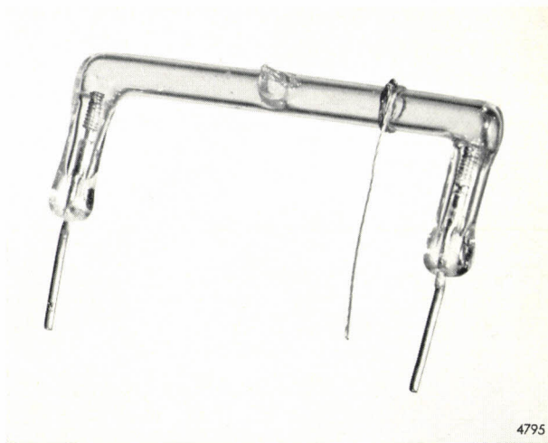
Fig. 15. Philips electronic-flash lamp, type OF 50 Ws (No. 3 in fig. 1 ).
