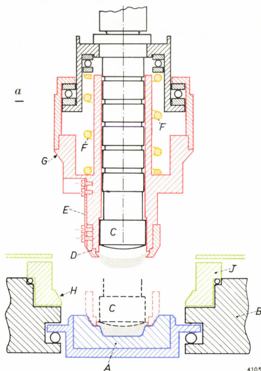
Fig. 5. a ) Schematic cross-section of a blow-head (red-black-yellow), a gob receiver (blue) and part of the turntable. A is the gob tray, mounted on a slide which moves in a radial groove in the turntable B . C blank plunger. D one of the claws which hold the glass (shaded) forced into them by the plunger. (The blanking position is represented by dashed lines.) E leaf-spring to which D is attached. F spring (yellow). G tapered edge of red part which, during the elongation of the parison, the blowing of the bulb and the ejection from the head, rests on the tapered edge H of the permanently rotating ring J (green). b ) The blown bulb is ejected by the plunger C , the red part of the head still resting on the ring J . In this operation the spring F is compressed somewhat more than in the blanking operation.
