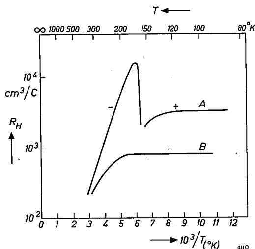
Fig. 2. Variation of Hall coefficient of (A) P -type and (B) N -type InSb with temperature. At temperatures below about 160 °K the Hall coefficient of sample (A) is positive. The high ratio of electron to hole mobility in indium antimonide causes the Hall coefficient to be negative at temperatures above 160 °K when it is a "mixed" conductor i.e. both electrons and holes are making a significant contribution to the conduction process. At higher temperatures both curves A and B approximate to the same straight line, which represents the intrinsic material.
