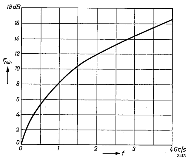
Fig. 1. Average F_{min} of the minimum noise figures in dB of 13 type EC 157 triodes, versus frequency.
