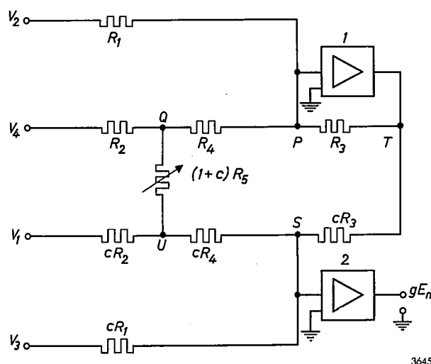
Fig. 12. Block diagram of the computing circuit for E_n . The probe potentials are applied to the terminals on the left. Amplifier 1 has a high gain, so that the potential of point P is effectively zero. The resistance values are such as to make V_S proportional to E_n . Since the network must not carry current, amplifier 2 is given a high input impedance. Only R_5 is dependent on the dimensions of the probes.
