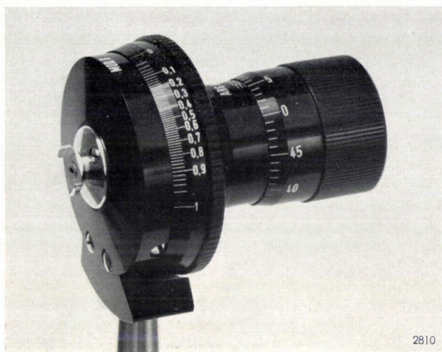
Fig. 16. Variable impedance as in fig. 15 , for 2 mm waves. The modulus and argument of the reflection coefficient can be read from separate scales. If reflection losses are eliminated, the absolute error in the modulus reading is less than 0.05.
