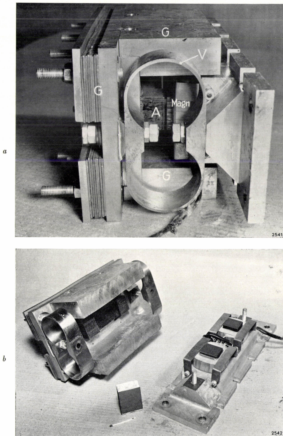
Fig. 12. a) Drive mechanism ready to be bolted to the foot of the tuning fork. Meaning of letters as in fig. 11. b) The mechanism dismantled. Right, the electromagnet with coils on base plate; left, the auxiliary mass with laminated armature and springs.
