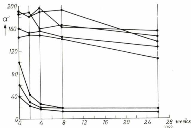
Fig. 9. Typical current amplification factor \alpha' versus time after encapsulation in dry silicone grease (lower three curves) and in moist silicone grease (upper five curves). The ambient temperature during the experiments was 50 °C, and 50 mW was dissipated in the transistors. The temperature of the germanium crystal was 85 °C. The transistors used were P-N-P types, electrolytically etched in KOH. \alpha' was measured at room temperature.
