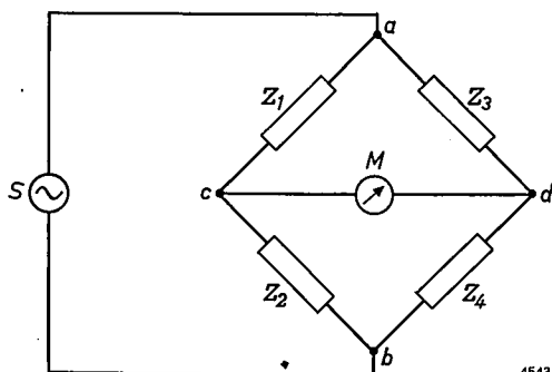
Fig. 7. Bridge circuit, consisting of impedances Z_1 , Z_2 , Z_3 and Z_4 . S voltage source. M detecting instrument.
