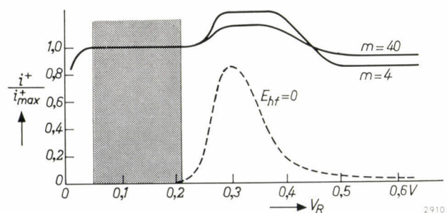
Fig. 8. Curves showing how the ion current i^+ depends on the positive potential V_R on the rings R. V_{CC'} = -25 V; V_{hf} = 1 V rms ; i^- = 1 \mu A; B = 0.5 Wb/m 2 . The dashed curve represents the ion current reaching the collector in the absence of an RF field. The shaded area is the operating region.
