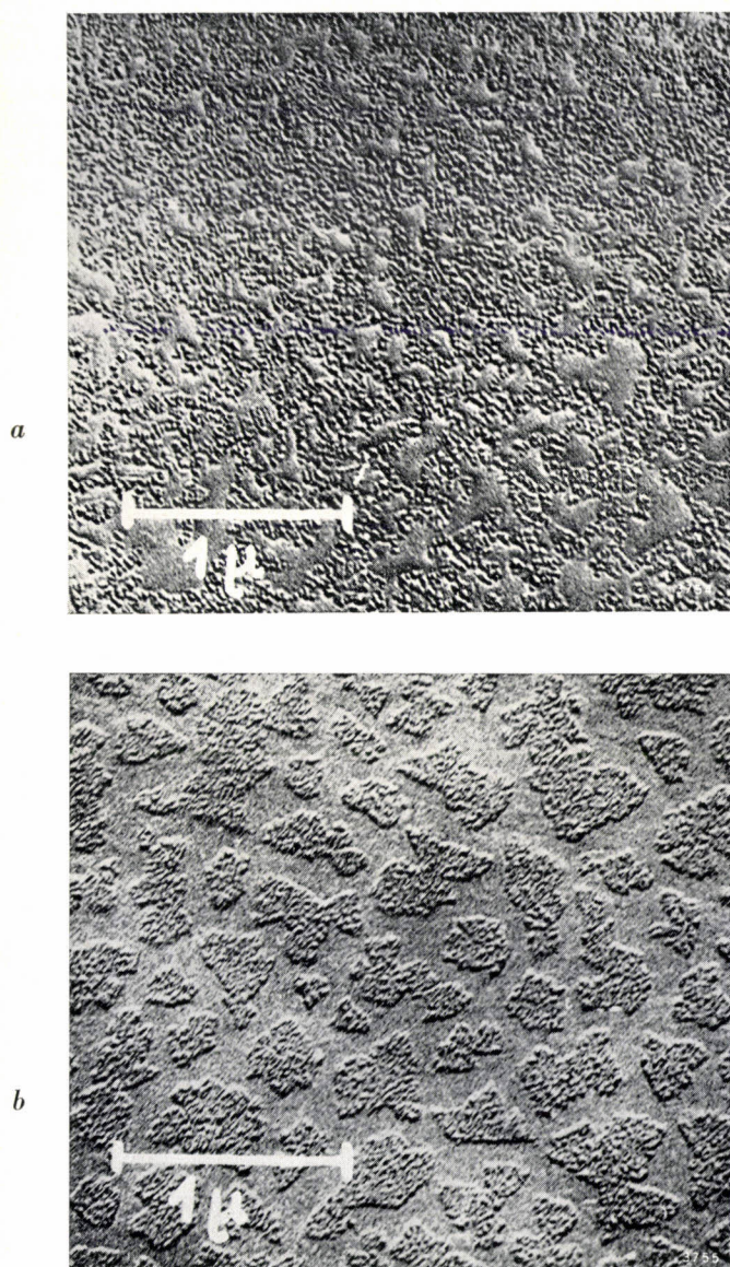
Fig. 10. Electron micrographs of sodium borate glass which is optically perfectly clear. a ) glass that has received no after-treatment, b ) glass heat-treated for 2\frac{1}{2} hours at 500^{\circ}\text{C} . (Taken from: W. Skatulla, W. Vogel and H. Wessel, Silikattechnik 9 , 51, 1958.)
