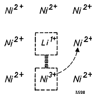
Fig. 9. The electric neutrality of a nickel-oxide crystal containing \text{Li}^{1+} ions is maintained by one of the surrounding Ni ions becoming trivalent. Due to the transference of an electron, the trivalence may move to any of the Ni ions that are immediate neighbours of the Li ion. This mechanism is proposed to explain the dielectric losses found at low temperature in impure or non-stoichiometric oxidic semiconductors.
