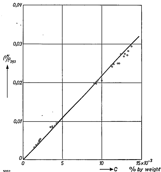
Fig. 3. The variation of the residual resistivity \rho'' (expressed as a fraction of \rho_{293} ) with the concentration C of carbon dissolved in iron. The relation between \rho'' and C is seen to be given by a straight line passing through the origin.
