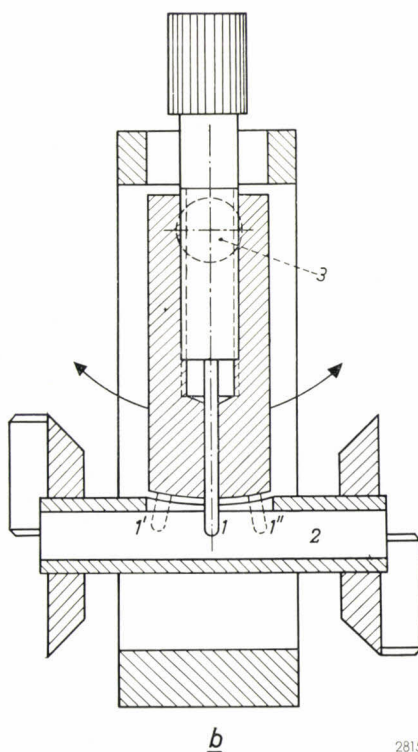
Fig. 4. Schematic representation of screw tuners. a) Sliding screw tuner. The dept of the stub 1 in the waveguide 2 can be adjusted by turning a screw, and its position along the waveguide can be adjusted between 1' and 1''. b) Pivoting screw tuner. Here too the stub 1 can be screwed in and out, but instead of sliding lengthwise it now pivots about spindle 3. The extreme positions are again 1' and 1''.
