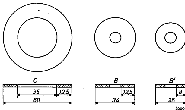
Fig. 5. Dimensions of the outer ring C and two kinds of shaft rings B and B' used in the tests.
