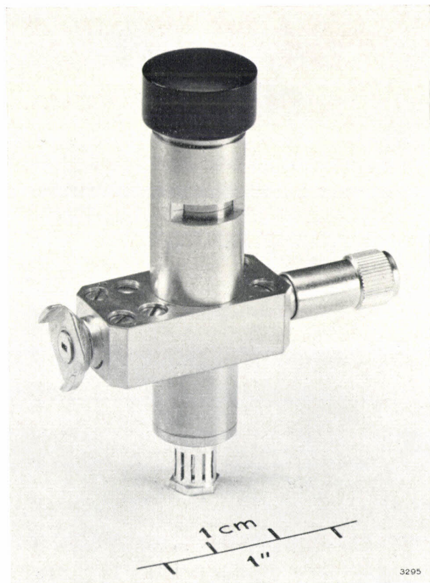
Fig. 1. Crystal detector for 2 mm waves. Left, claw flange, right, shorting plunger. The differential screw which is used to bring the silicon crystal into contact with the catwhisker is situated beneath the black cap; the displacement can be monitored through the window. Below: the coaxial connection for the millivoltmeter. The sensitivity is better than 10 mV per mW.
