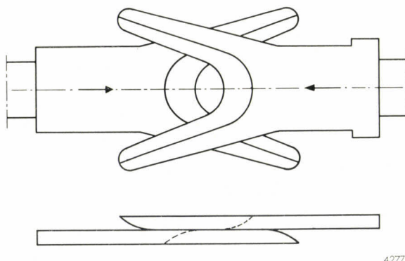
Fig. 3. Shears for cutting the viscid stream of glass issuing from underneath the furnace into “gobs” (schematic). The two V-shaped knives slide one over the other in the direction of the arrows.
