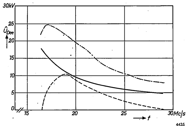
Fig. 12. Solid curve: amplitude of the voltage \hat{U}_{dee} at the dee mouth, calculated as a function of frequency f . Dashed curve: the ideal amplitude programme corresponding to the frequency variation shown in fig. 10. Dot-dash curve: actual variation of voltage amplitude.
