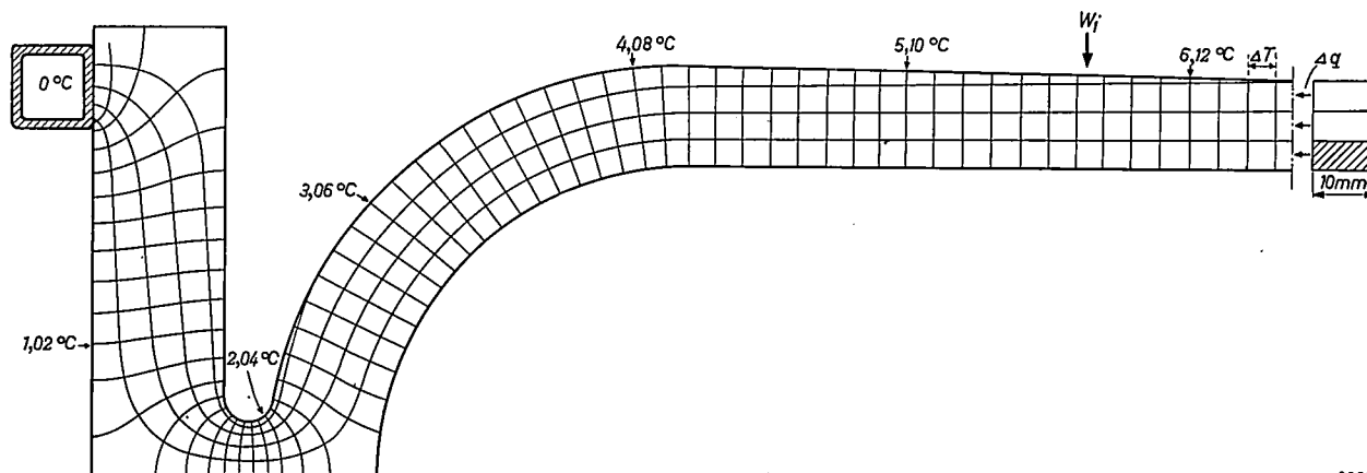
Fig. 20. Streamlines of heat-flow and equal-temperature contours in the profile of a blade of the tuning fork (only the curved section is reproduced, the temperature variation in the straight section being almost linear). In each stream tube (shown hatched in cross-section) a power \Delta q flows of 0.14 W. Since only the temperature differences are important here, the temperature in the cooling-water pipe (top left) is assumed to be 0 °C.
