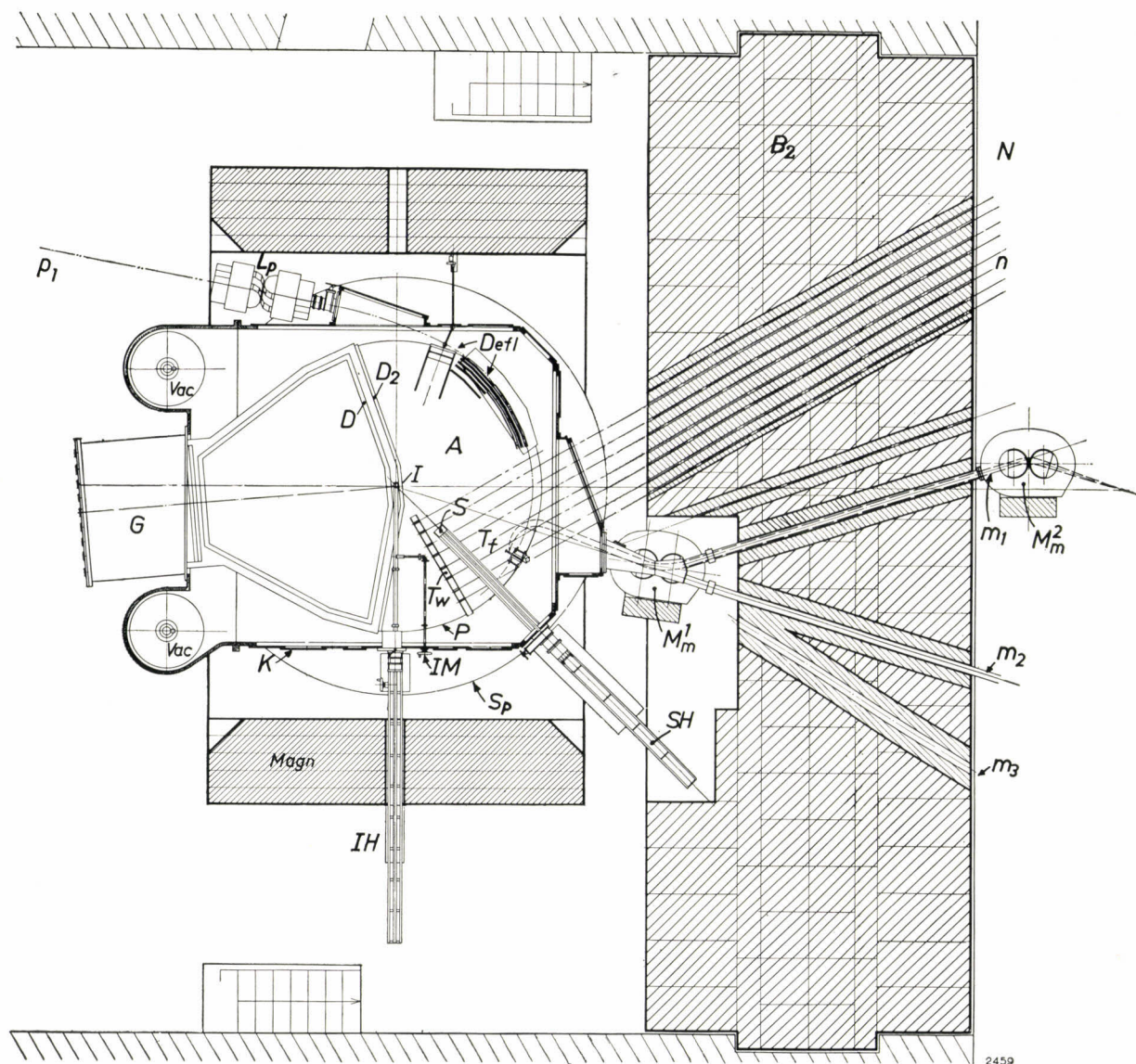
Fig. 7. The accelerating space A in the vacuum chamber K , with channels through the protective wall B_2 leading to the neutron experiment room N . Only one of the dee electrodes ( D ) is connected to the radio-frequency system; the second is earthed and is therefore a simple slotted strip ( D_2 ), leaving the whole of the right half of the chamber free for target assemblies. I ion source attached to arm IH and with adjusting mechanism IM . T_w eight "flip targets", which can be set upright for producing neutrons of different energies (beams n ). S probe fitted to arm SH , one purpose of which is to measure the intensity of the proton beam at various distances from the centre. Defl magnetic channel with devices for extracting the protons from the accelerating chamber. L_p lens for strong focusing of the extracted proton beam p_1 . T_f Fermi trolley, i.e. universal target, which can be moved around the outermost proton orbit, for the production of mesons; in the position illustrated, negative pions are extracted by the deflection magnets M_m^1 and M_m^2 . The meson beams are m_1 , m_2 , m_3 . Magn yoke of cyclotron magnet. P magnet pole. Sp energizing coil. Vac pumps. G radio-frequency source and tuning-fork modulator.
