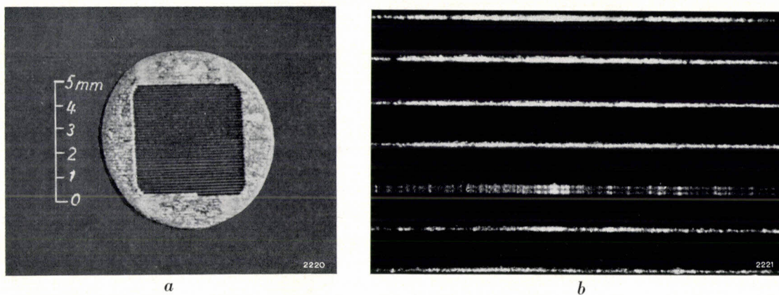
Fig. 20. a) Frame grid of a tube for very high frequencies. b) Picture under the microscope when the grid was made to vibrate at the resonance frequency of one of the wires (37 000 c/s).
