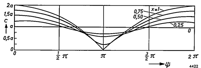
Fig. 8. Amplitude modulation of vector c (fig. 5). The variation of the amplitude c is shown as a function of the angle \psi between a and b , for various values of the signal ratio x = b/a .
