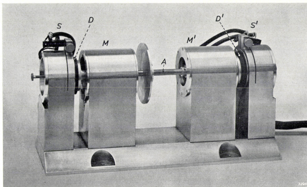
Fig. 11. Shaft A with magnetic bearings M and M' , ferroxcube disks D and D' and axial stabilizers S and S' .
