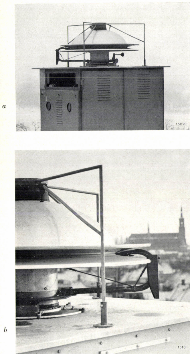
Fig. 8. a) Mounting of the antenna on the housing containing the radar transmitter and receiver. b) Close-up view of antenna.
