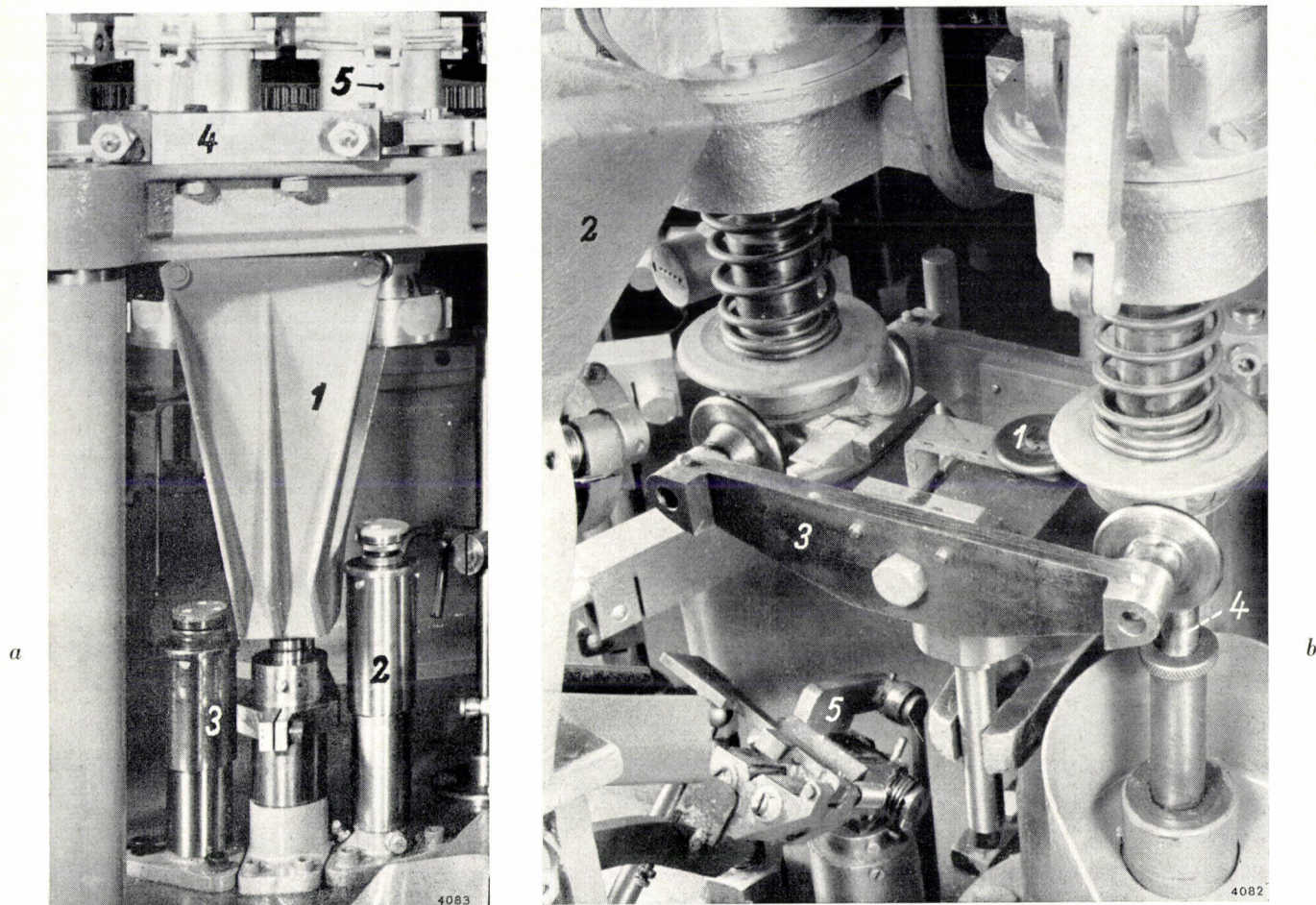
Fig. 18. a ) Detail of 32-head machine for working long sections of glass tubing (in course of development). In the part shown, the tubes are being adjusted to the correct height. This is done here in two stages. 1 chuck opener. 2 first glass-gatherer. 3 second glass-gatherer. During the glass-gathering operations the chucks are not in rotation; this is achieved by the cam 4 actuating the lever 5.
