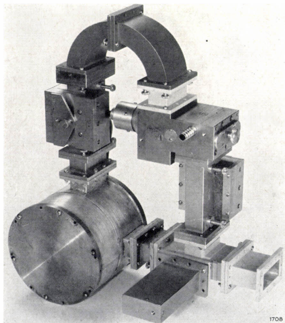
Fig. 9. a) Oscillator for 4000 Mc/s fitted with an EC 157, built on the principle of fig. 8a. b) Similar oscillator, but for 6000 Mc/s and fitted with a 5 cm, 1 W triode. Both oscillators, a and b , are reproduced on the same scale.
