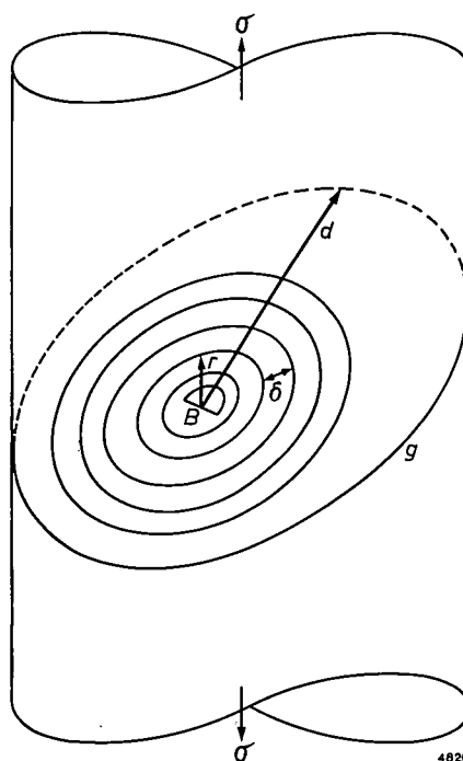
Fig. 14. Model representing the creep process in germanium. A cylindrical crystal is subjected to a stress \sigma causing the source B on the slip plane g to send out dislocation loops separated by intervals \delta . The radius r of each loop increases proportionally with time. The dislocation density rises until the radius of the first ring is equal to d , and the dislocations begin to leave the slip plane at the other side of the crystal. A stationary state then sets in.
