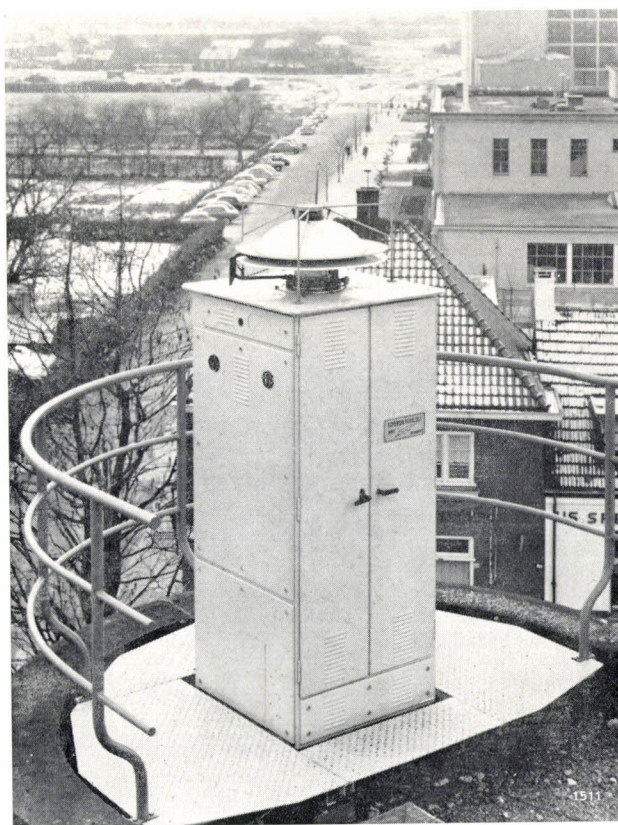
Fig. 9. Experimental radar installation with fast-scanning antenna system of the type described, on the roof of Philips Research Laboratories at Eindhoven.
