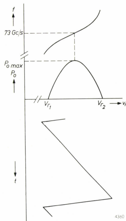
Fig. 11. The repeller voltage v_r of the klystron in fig. 9 has a sawtooth waveform. The klystron oscillates between the limits V_{r1} and V_{r2} . The output power P_0 and frequency f vary as shown. At P_0 = P_0 \text{ max} the value of f must be approximately 73 Gc/s.
