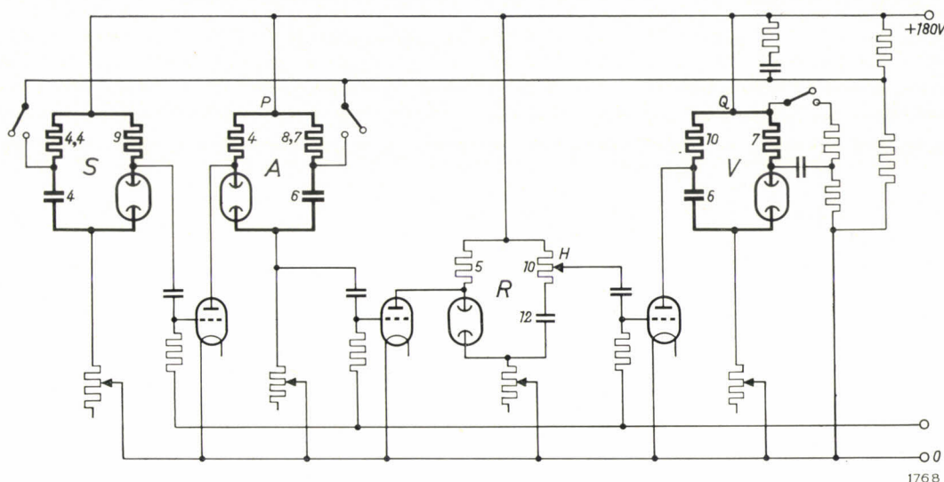
Fig. 8. Circuit simulating the functioning of the heart. Resistance values in k\Omega , capacitances in \mu F . The three circuits S , A and V , each of which can enter into relaxation oscillations and which are coupled in a special way, represent respectively the sinus venosus, the auricles and the ventricles. R is a delay system which simulates the transit time of a stimulus through the bundle of His. The ignition of each of the neon lamps in S , A and V corresponds to a systole of that part of the heart. The coupling between auricles and ventricles can be varied with the potentiometer H (Erlanger's experiment). Electrocardiograms can be made by recording the current in one of the leads from point P or Q .
