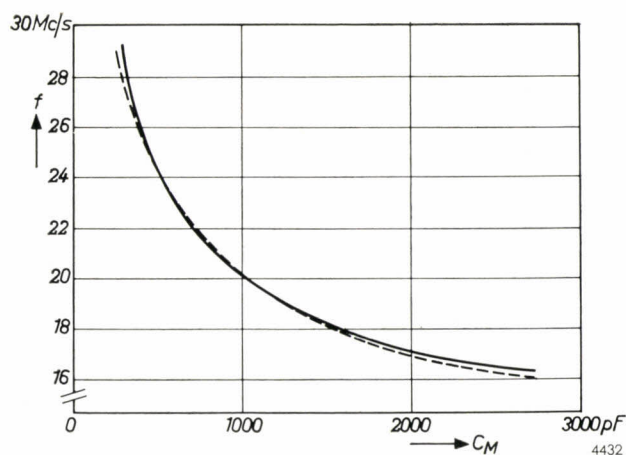
Fig. 9. Measured variation of the natural frequency f of the resonator as a function of tuning-fork capacitance C_M . The dashed curve represents the calculated variation.
