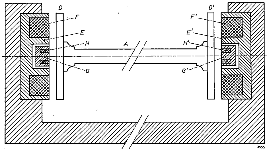
Fig. 10. System for stabilizing the shaft in an axial direction. D and D' are ferroxcube disks which can be attracted by electromagnets E and E' , excited by coils F and F' . The self-inductance of the coils H and H' on the cores G and G' is dependent upon the distance to the disks D and D' . The magnetic bearings themselves are omitted here.
