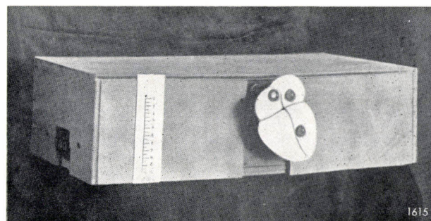
Fig. 9. Photograph of the heart simulator. The three neon lamps of the circuits S , A and V (see fig. 8) are mounted on the three corresponding parts of the anatomical representation of the heart.
