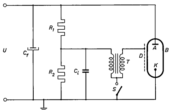
Fig. 2. Basic circuit for an electronic-flash lamp. The main capacitor C_f is charged to a DC potential U . B envelope, A anode, K cathode and D trigger electrode. R_1 - R_2 voltage divider for the triggering voltage. C_i capacitor for trigger pulse. S initiating contact, normally built into the camera and synchronized with the shutter. T trigger-pulse transformer.
