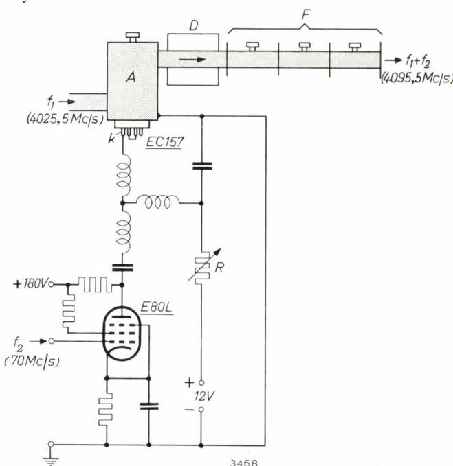
Fig. 11. Circuit 15 for an EC 157 used as a mixer for transferring the modulation of an IF signal ( f_2 ) to an RF signal ( f_1 ). A amplifier. D isolator. F three-stage filter. k cathode lead of EC 157.
