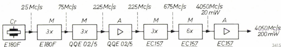
Fig. 5. Block diagram of a local oscillator 15) for microwave radio-link relay station. Cr crystal oscillator. M frequency multipliers, the last two fitted with EC 157 triodes. A amplifiers.
