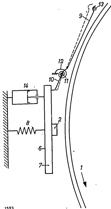
Fig. 8. Illustrating the method of maintaining a constant distance of about 1 \mu between the magnetic wheel 1 and the writing-reading head 2. 6 arm with pivot 7. 8 compression spring. 9 vane, with arm 10 and pivot 11. When the wheel is stationary the coil spring 12 forces the vane against the stop 13; the arm 10 then prevents the spring 8 from pressing the head against the wheel. When the wheel is turning at full speed the air stream around the wheel pushes the vane 9 outwards (to position of dashed line) against the action of the coil spring 12; arm 10 then releases arm 6, and spring 8 pushes the head towards the wheel. The air film dragged round by the wheel forms an air cushion on which the head rides at a constant distance of about 1 \mu from the wheel. 14 oil damping.
