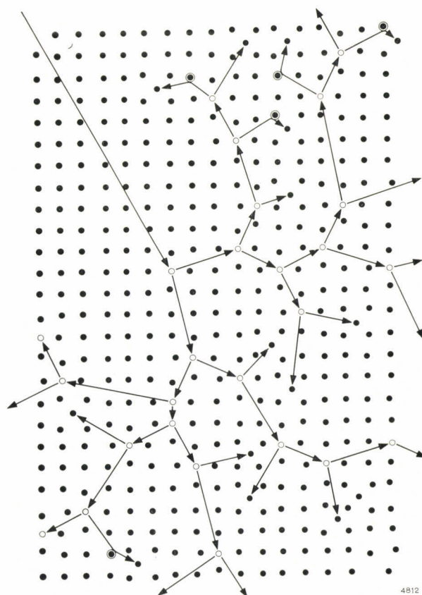
Fig. 5. Schematic representation of the imperfections that may be produced by irradiating a crystal with high-energy neutrons (after D. S. Billington, Scientific American 201 , No. 3, p. 200, 1959). Vacancies (open circles) and interstitial atoms are formed by sequences of collisions in cascade.
