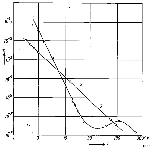
Fig. 3. The characteristic time \tau of a paramagnetic relaxation increases steeply as the temperature falls. The figure gives a log-log plot of \tau (in seconds) versus temperature, as measured on two substances: 1: \text{Gd}_2(\text{SO}_4)_3 \cdot 8\text{H}_2\text{O} ; measured at 2.6 \times 10^5 A/m; 2: \text{CrK}(\text{SO}_4)_2 \cdot 12\text{H}_2\text{O} ; measured at 3.2 \times 10^5 A/m.
