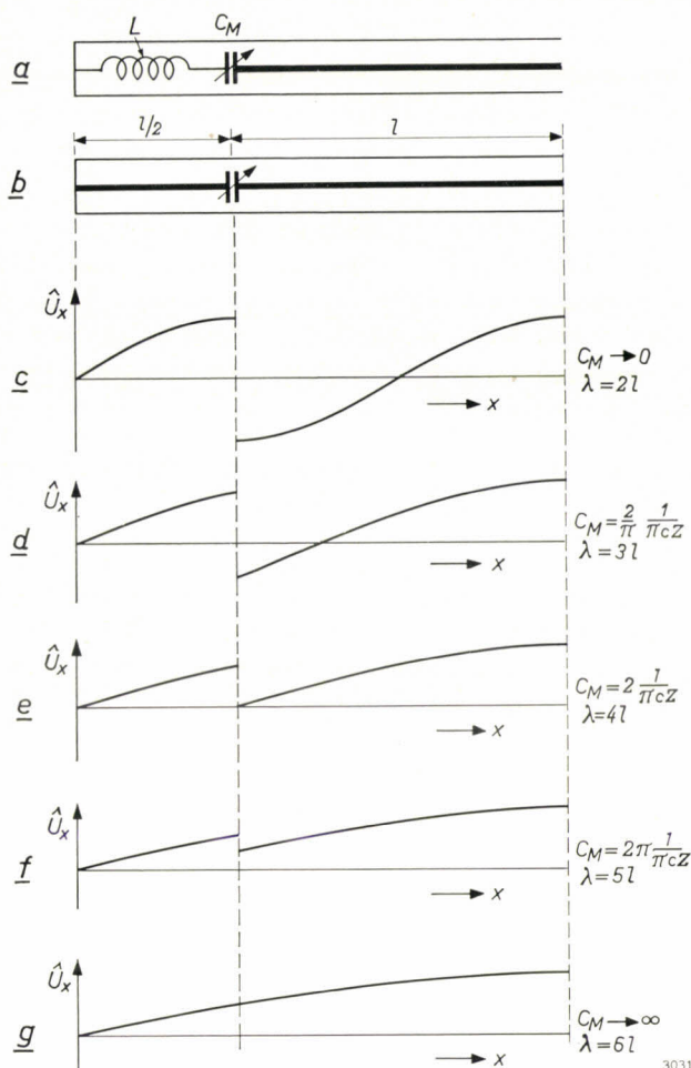
Fig. 3. a ) The modulating capacitor is turned into a series resonant circuit by the addition of an inductance L . b ) This inductance is in reality a short-circuited section of line (stub). c ) to g ) Voltage distribution on the resonator thus formed, at different values of capacitance C_M . Cases ( d ) and ( f ) roughly correspond to the extreme values attainable with the tuning-fork capacitor.
