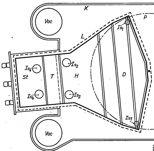
Fig. 13. Construction of the resonator and its positioning in the cyclotron. D dee with reinforcement ribs, supported at the two points Is_1 . H dee stem, suspended at the two points Is_2 . T tuning fork. St stub, suspended at the two points Is_4 . L outer conductor of resonator. K accelerating chamber. Vac pumps. p outermost proton orbit.
