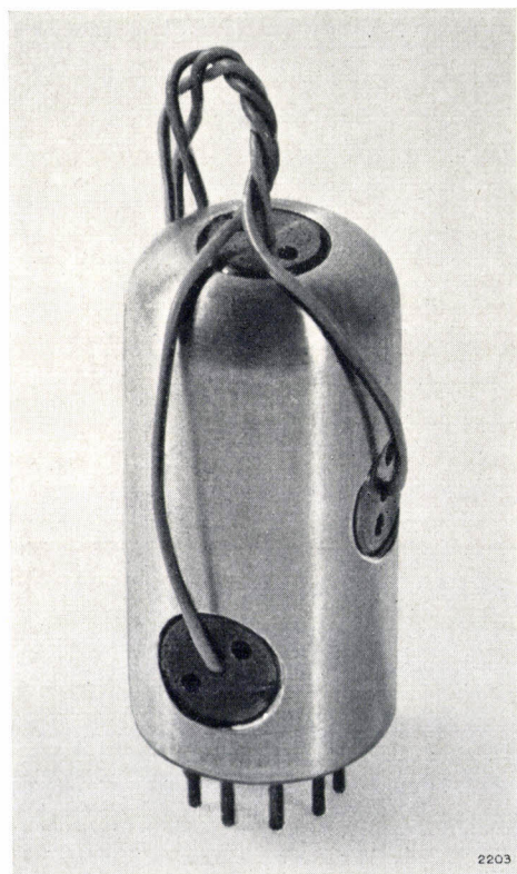
Fig. 2. Combination of three vibration pick-ups, used for measuring the vibrations to which tubes are subjected in electronic equipment. The whole assembly can be fitted in a tube holder in place of a tube.
