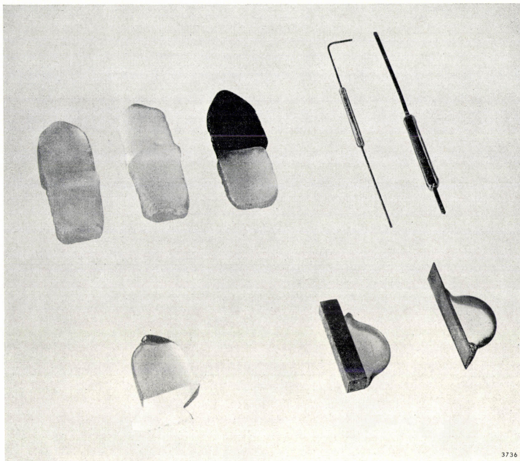
Fig. 2. Various test seals. Top left: glass-to-glass, viz. translucent, opalescent and black glass sealed to translucent glass. Top right: bead seals. Bottom left: glass-to-ceramic. Bottom right: plate seals. Roughly actual size.
