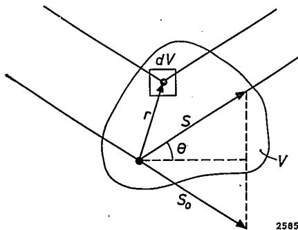
Fig. 5. Determination of the reflection condition for a density wave. \mathbf{S}_0 and \mathbf{S} are unit vectors denoting respectively the directions of incidence and scattering of an X-ray beam, two rays of which are shown. \mathbf{r} is the vectorial distance between two scattering points, dV is a volume element of the total volume V , and \theta is the semi-angle of reflection.
