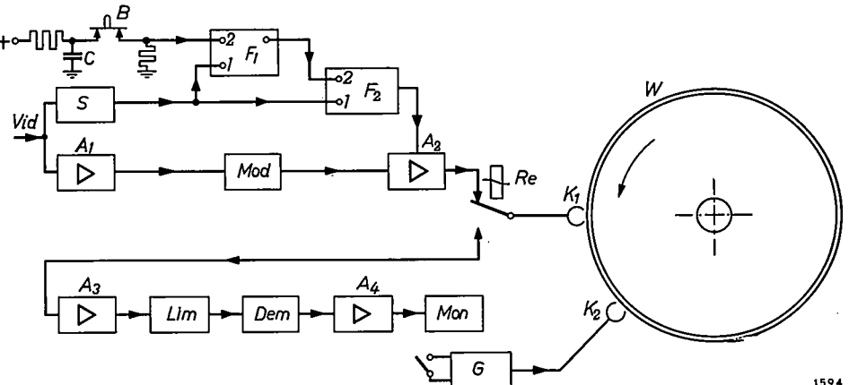
Fig. 9. Block diagram of the circuit for writing and reading a single frame. Vid video-signal input. A_1 video amplifier. Mod modulator, in which the video signal modulates a carrier wave in frequency. A_2 recording amplifier. Re write-read relay. K_1 write-read head. W wheel store. S circuit which separates picture-synchronizing signals — “sync pulses” — from video signal. F_1 and F_2 bistable flip-flops, with inputs 1 and 2. B push-button, which, by discharging capacitor C, produces the “display” pulse. A_3 read amplifier. Lim limiter. Dem demodulator (frequency detector). A_4 video amplifier. Mon monitor. K_2 erasing head. G erasing-current generator.
