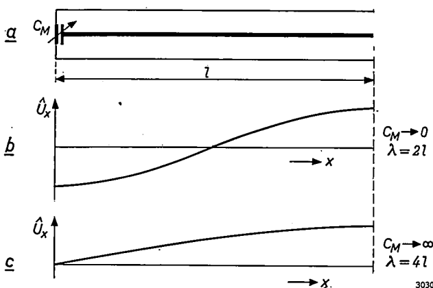
Fig. 2. a) Simplest form of a coaxial transmission line coupled to modulating capacitor C_M . b) and c) At the limiting values C_M = 0 and C_M = \infty , a standing wave of \frac{1}{2}\lambda and \frac{1}{4}\lambda , respectively, is set up in the resonator (the voltage amplitude U_x is plotted against distance x ).
