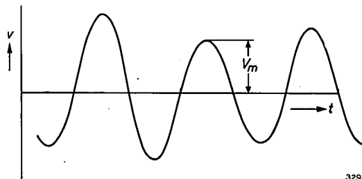
Fig. 4. Illustrating what is meant by the "instantaneous peak value" V_m of the filtered noise v . The quantity V_0 , which occurs in (14), is the r.m.s. value of V_m .
