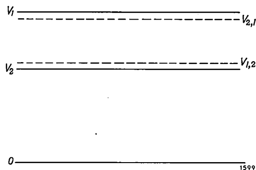
Fig. 14. V_1 potential of point K (fig. 13) in stable state 1; V_2 idem in state 2. V_{1,2} value which v_{C1} must reach to cause state 1 to change to state 2; V_{2,1} idem for transition from 2 to 1.
