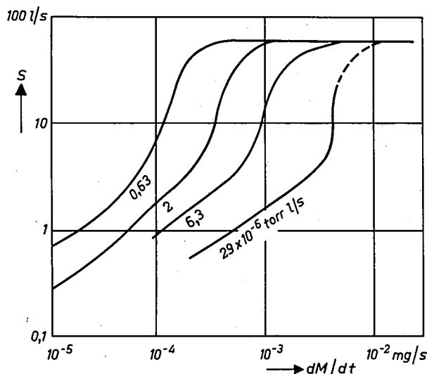
Fig. 2. Pumping speed S in l/sec as a function of evaporation rate dM/dt in mg/sec, for various influx rates of CO in torr.litre/sec.
