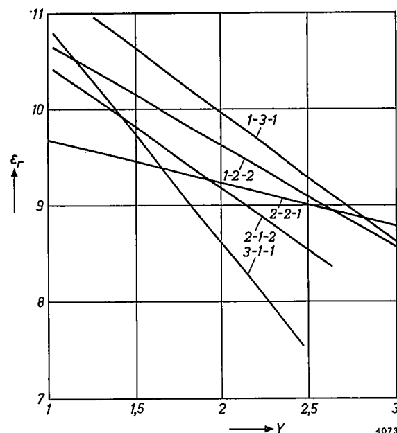
Fig. 9. Relative dielectric constant \epsilon_r of K_2O - CaO - SrO silicate glasses as a function of Y , measured at 1.5 Mc/s. The mole fractions of the metal oxides are indicated in the same way as in fig. 7. No inversion occurs. This is due to the fact that the dielectric constant is not governed by the coherence of the structure, but solely by atomic properties.
