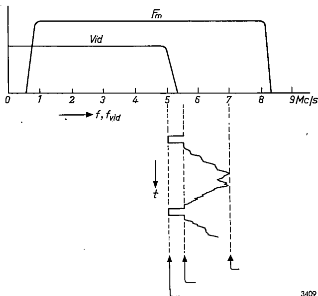
Fig. 4. Vid frequency range of the video signal for a television picture with 625 lines. Fm frequency range of the signal to be recorded, whose instantaneous frequency is 7 Mc/s in the brightest white, 5.5 Mc/s in the black, and 5 Mc/s in the "blacker-than-black" (peak of sync signals).
