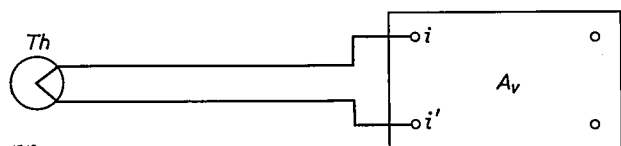
Fig. 6. Thermocouple Th , connected by a long twin-cable to the input terminals i and i' of a difference amplifier A_v .
